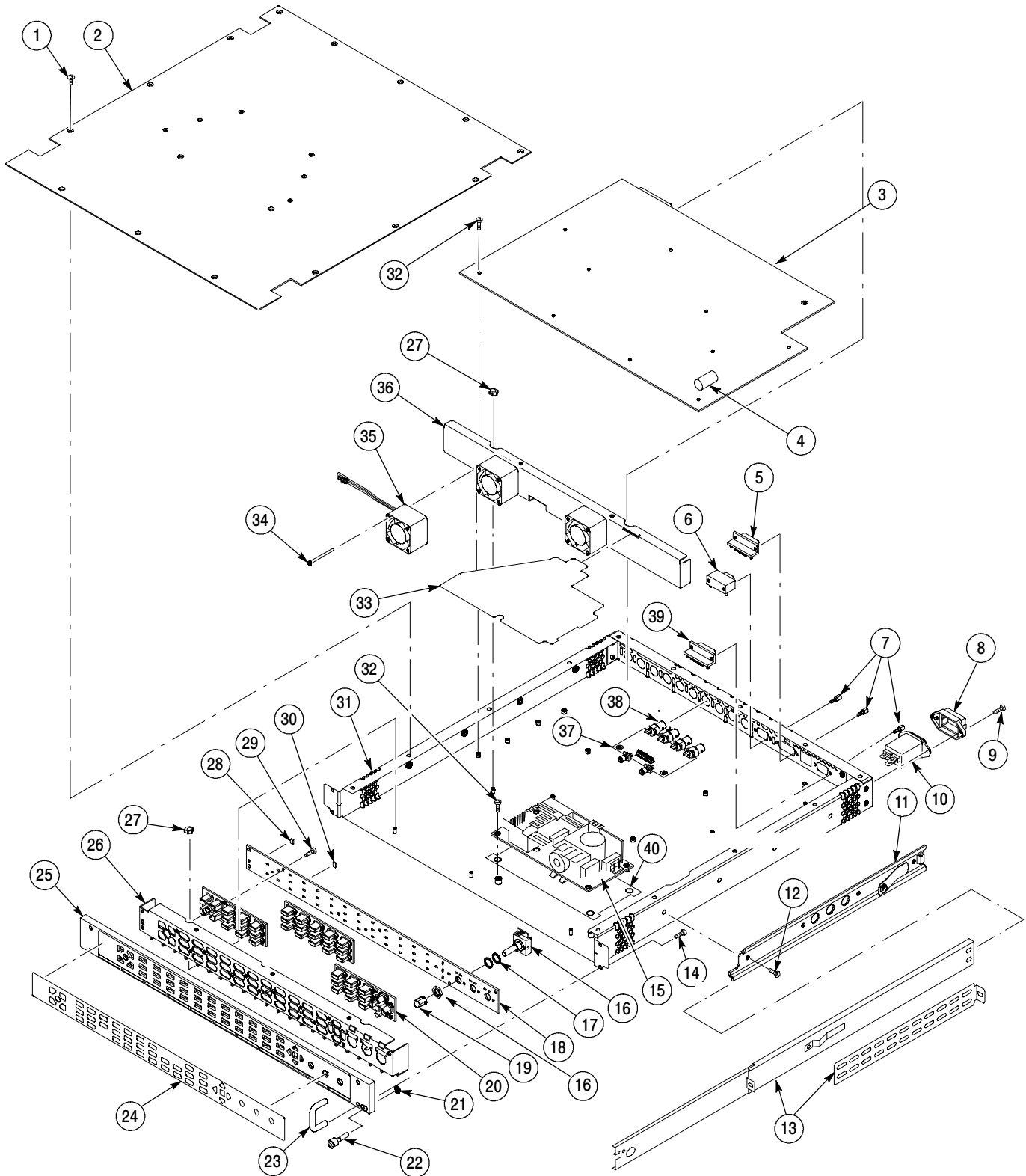
Figure 5-1: Replaceable mechanical parts, WR7100
