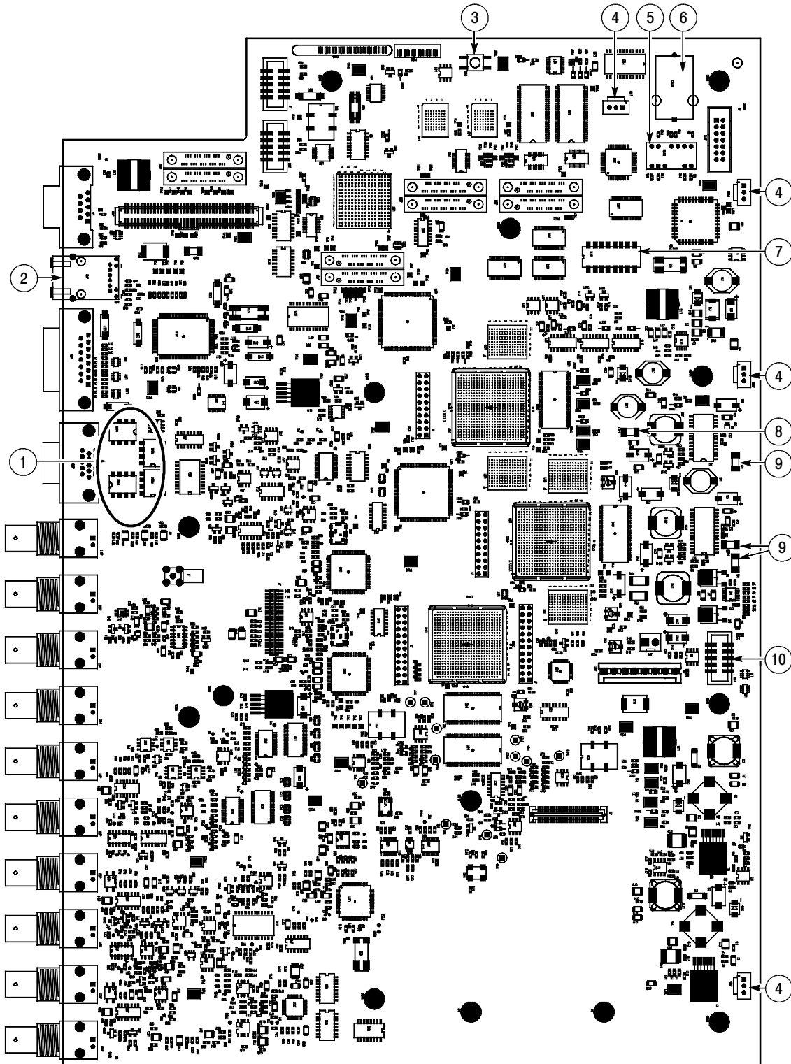
Figure 5-5: Main board replaceable components and connectors, WVR7100 (B020100 and later) and WVR6100 (all)
