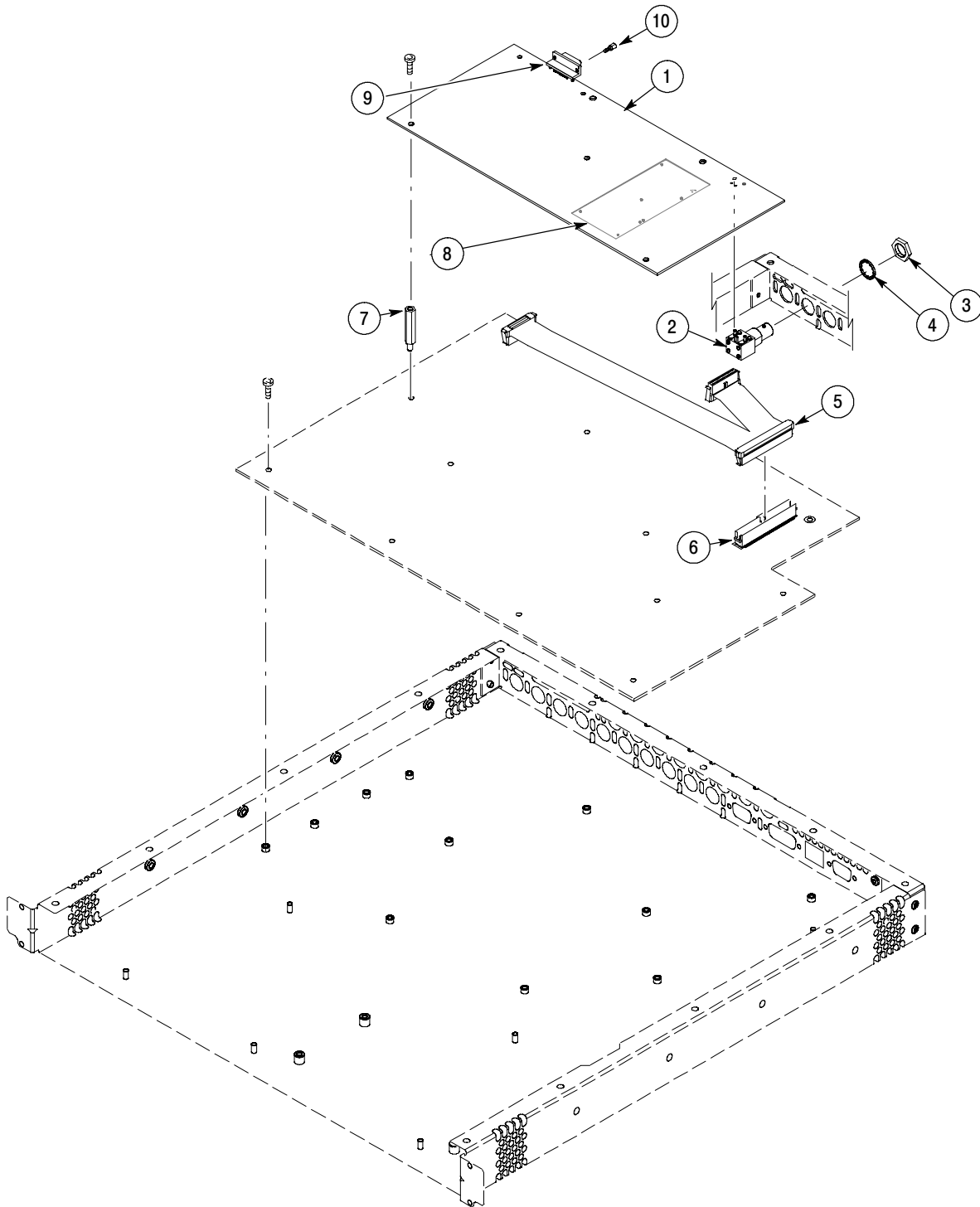
Figure 5- 6: Audio DA and DG Options boards and connectors
