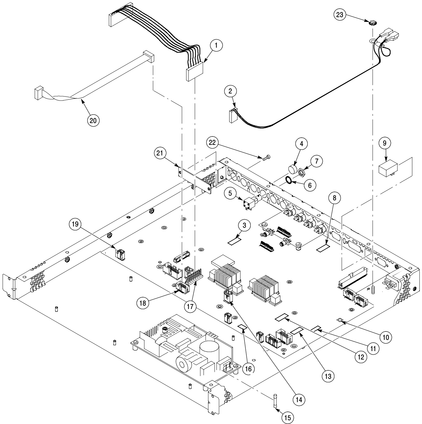
Figure 5-3: Replaceable cables, connectors, and other mechanical parts, WVR6100 and WVR7100
